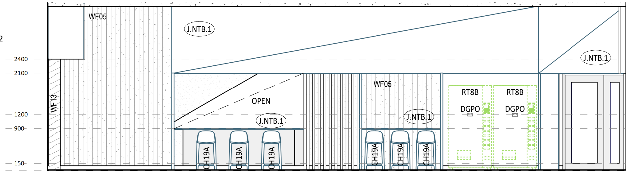
3 ELEVATION DETAIL 60-033 1 : 50
