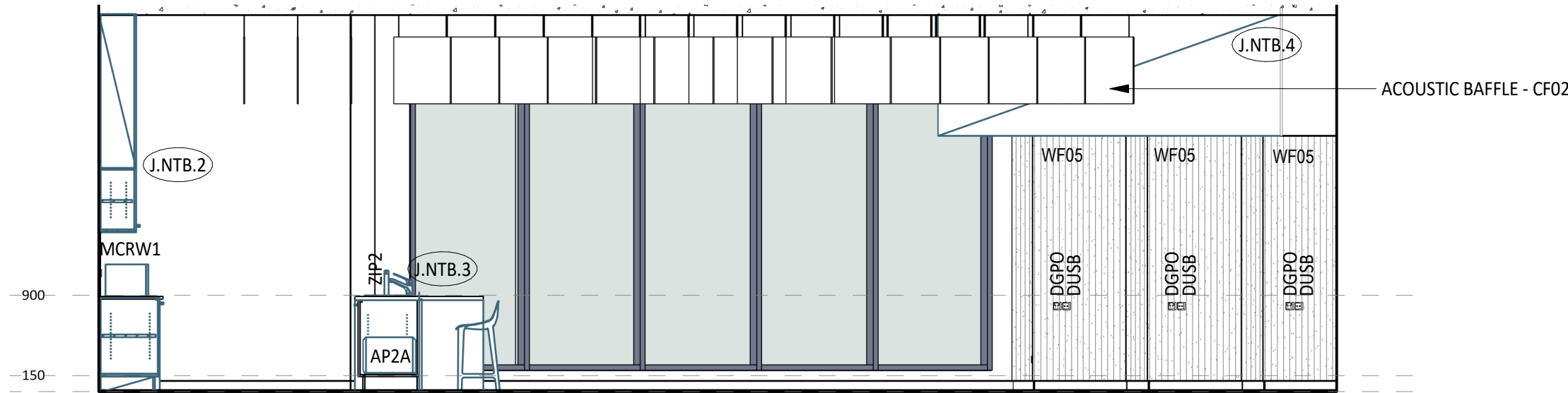
2 ELEVATION DETAIL 60-033 1 : 50
