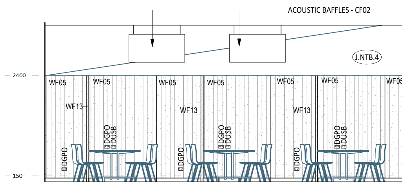
4 ELEVATION DETAIL 60-034 1 : 50
