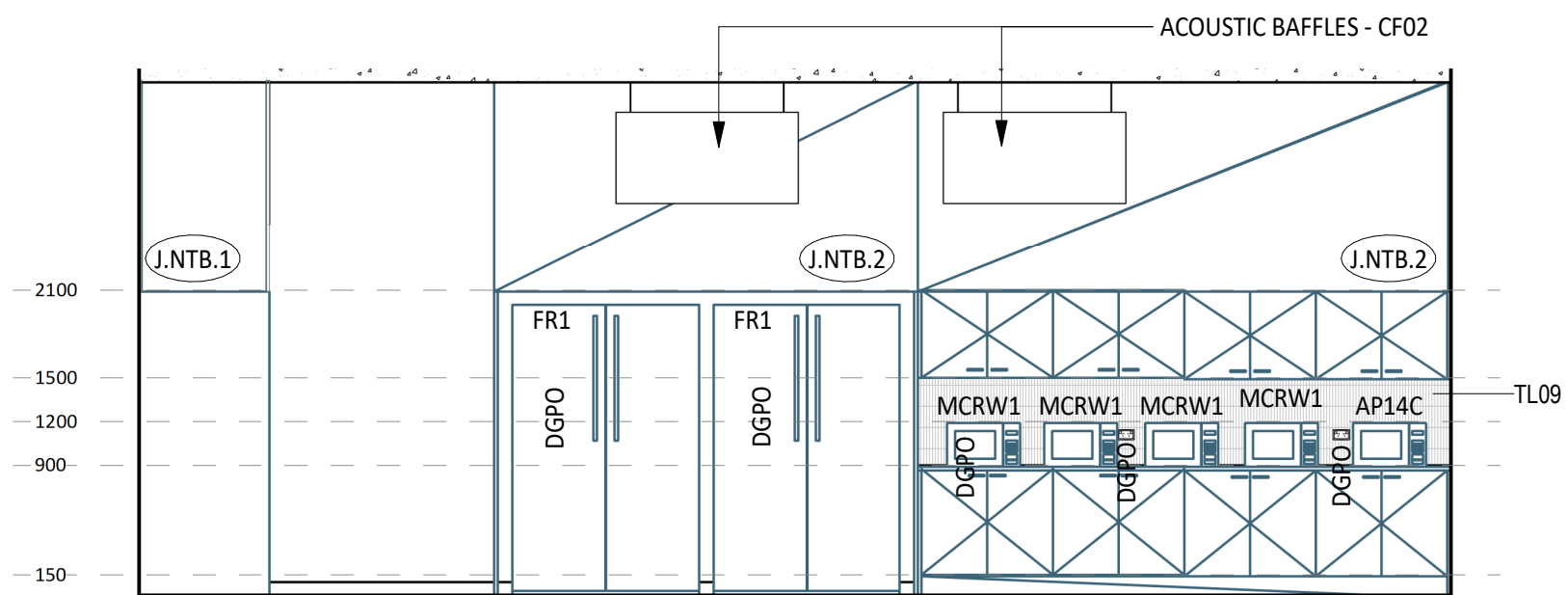
1 ELEVATION DETAIL 60-034 1 : 50
